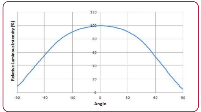
Radiation Diagram for all "XO" product
